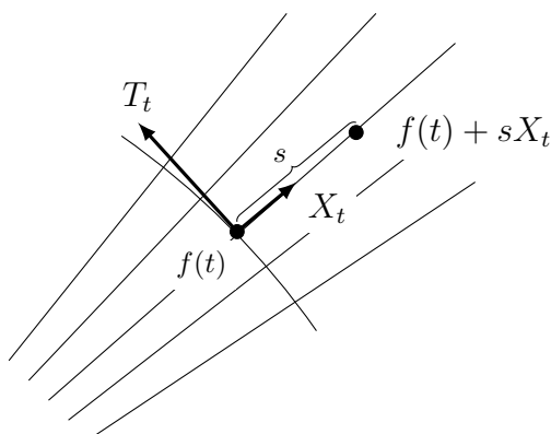
Figure 2.5: Ruled Surface
