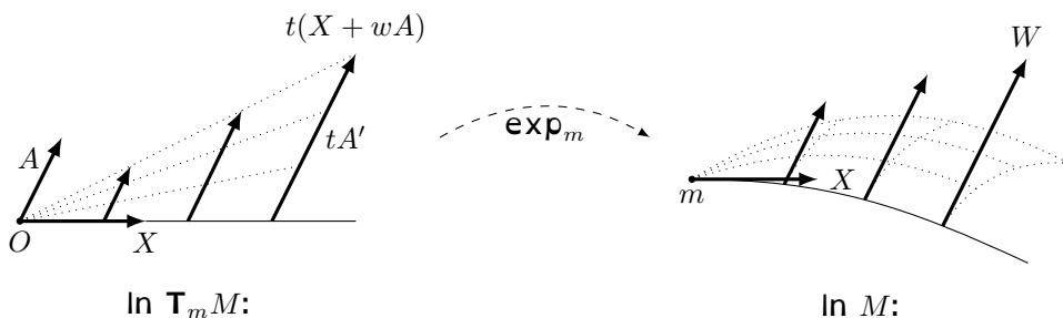
Figure 10.1: Jacobi Field
