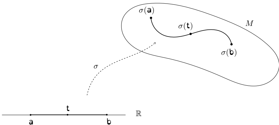
Figure 1.3: A Curve
