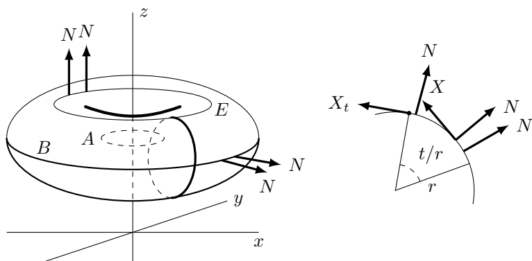
Figure 2.4: The Torus
