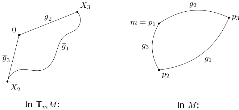
Figure 10.6: Geodesic Triangle
