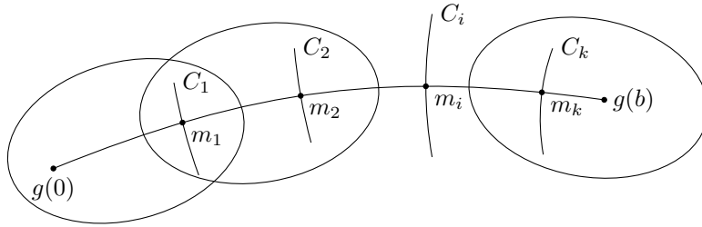
Figure 10.5: Cross Manifolds
