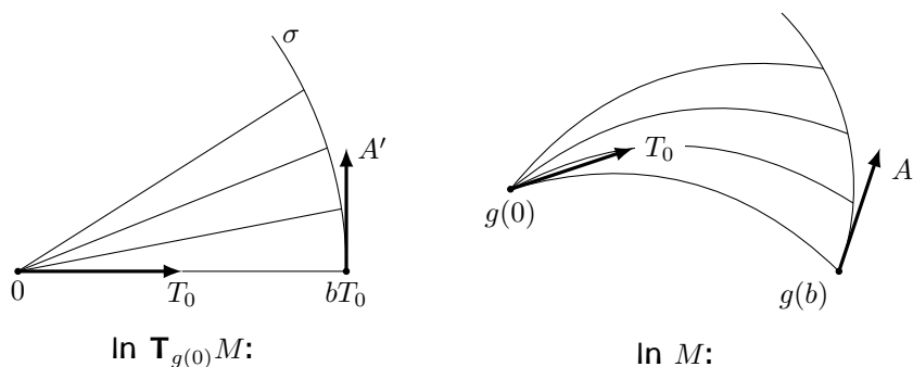
Figure 10.3: Comparing Geodesics
