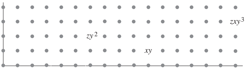
The E_\infty -term
