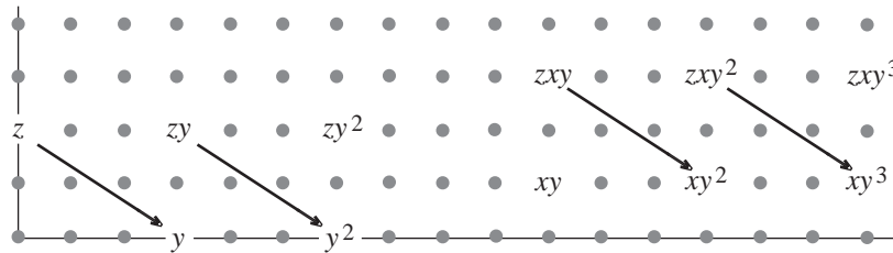
The E_3 -term
