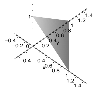
The standard topological 2-simplex \Delta^2 \in \mathbf{R} .
